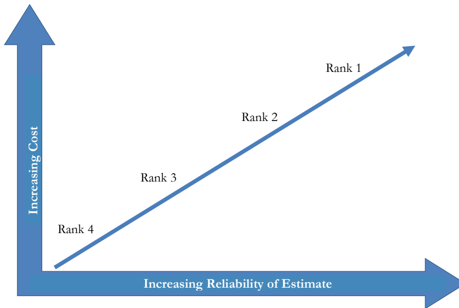
Figure 2.2 Emission estimation methodology rankings
