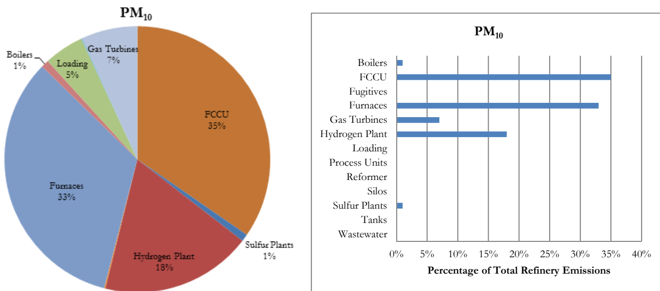
Figure 8.3.1 Example source category PM 10 emission summary in graphic forms
